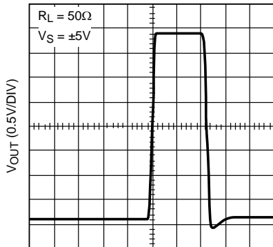
TIME (20 ns/DIV) Figure 17.
